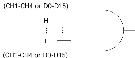
Figure 5-6 Pattern Trigger
