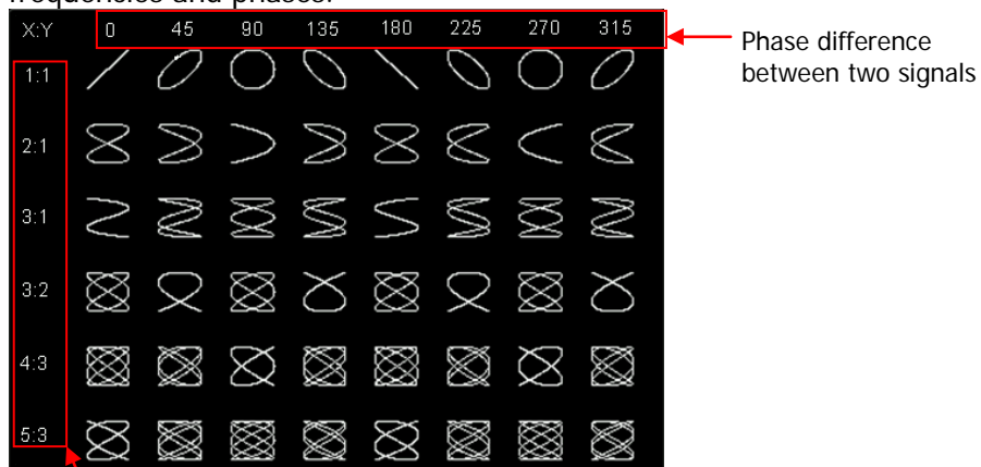
Figure 6-9 Lissajous Schematic Diagram
